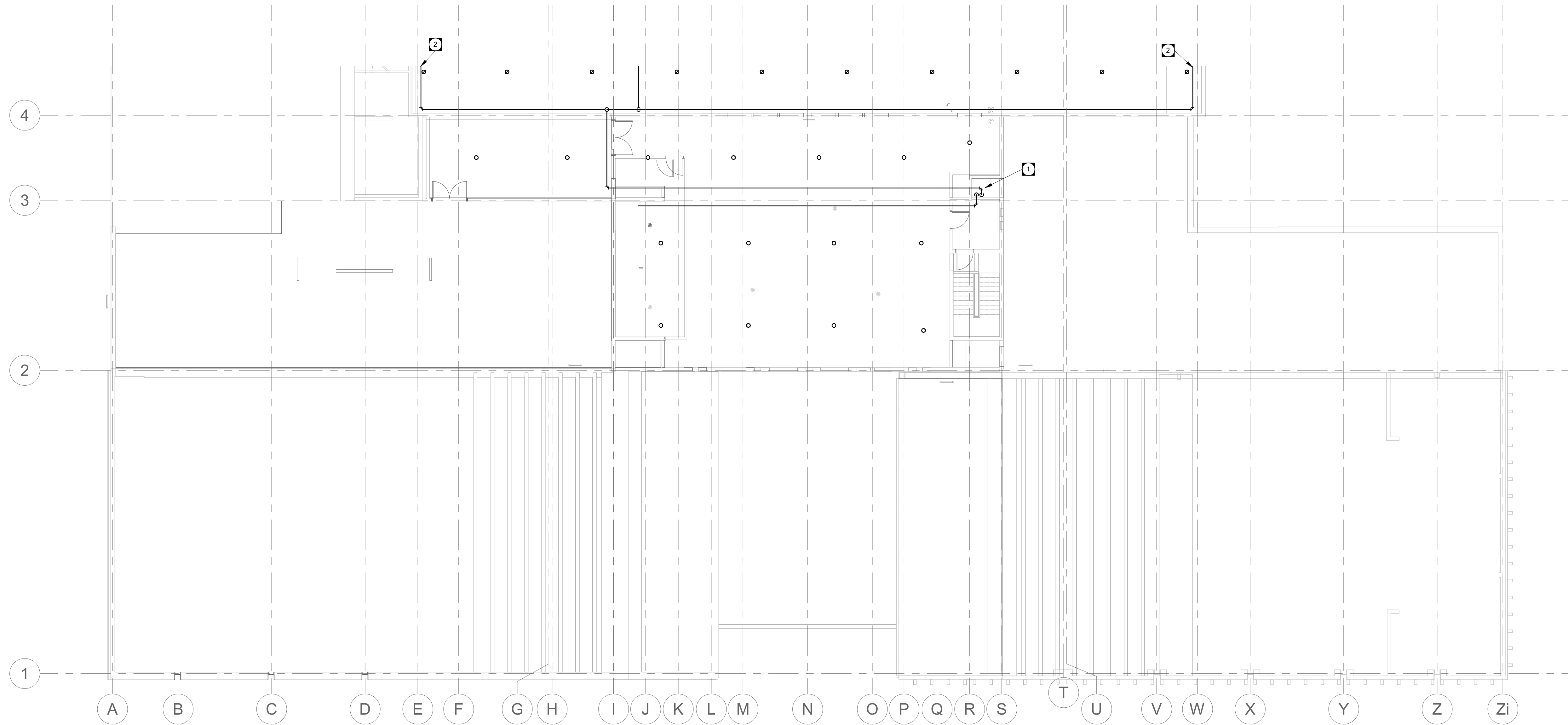
LEVEL 2 - FIRE PROTECTION RENOVATION 1 3/32" = 1'-0" MF2.2
